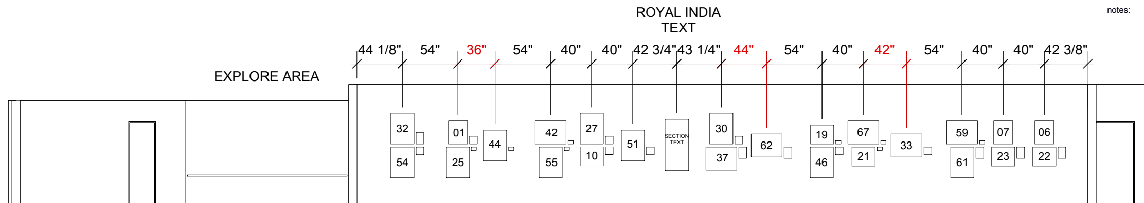
NORTH SECTION / NORTH WALL SCALE: 1/8" = 1'-0"
