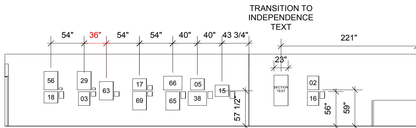
EAST SIDE / EAST WALL SCALE: 1/8" = 1'-0"
