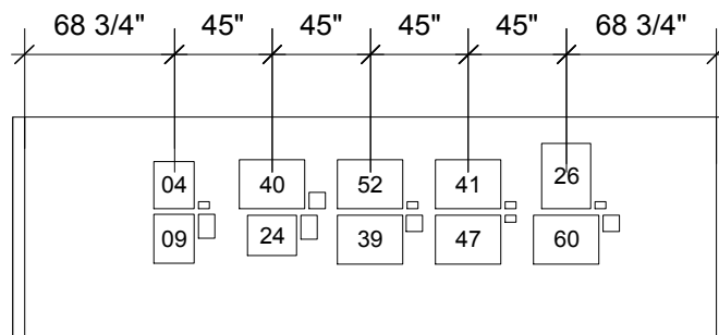
NORTH SECTION / NORTH WALL SCALE: 1/8" = 1'-0"
