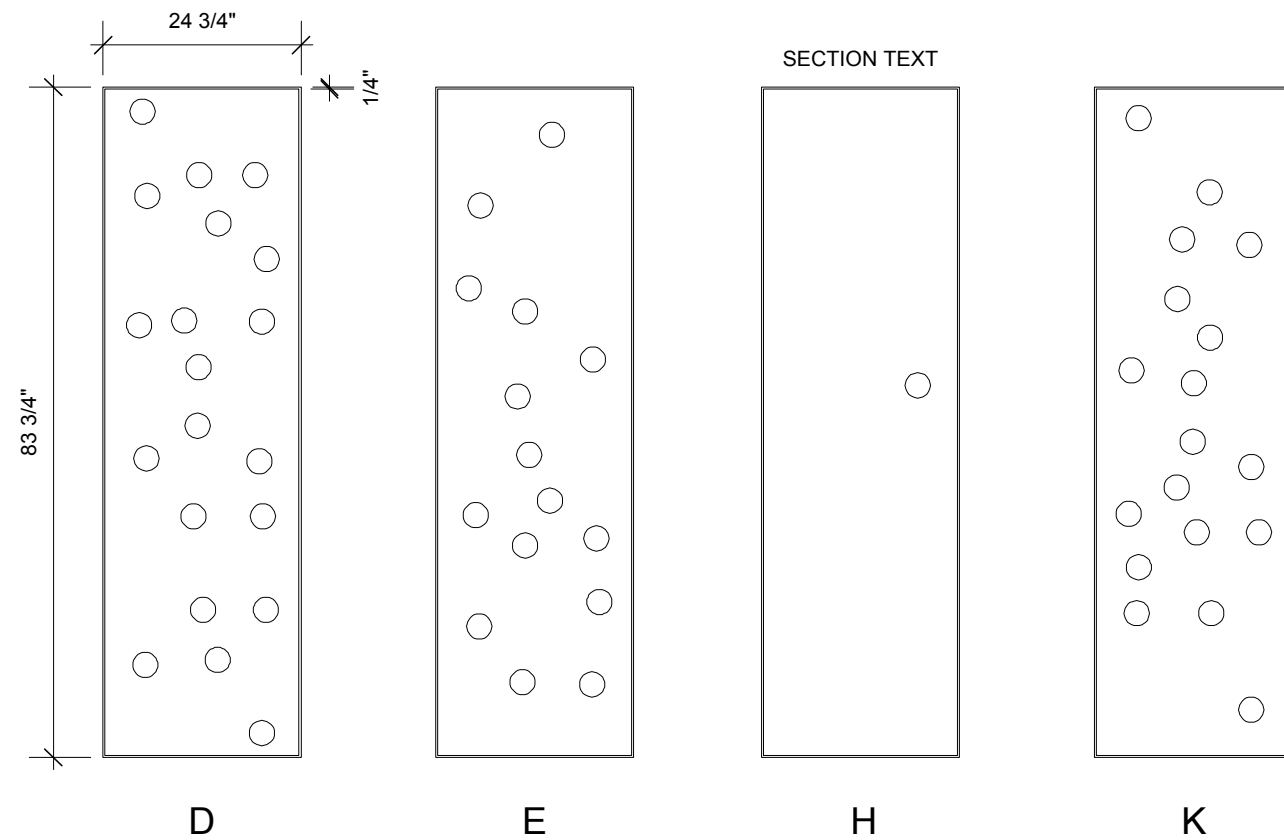
4 SMALL PANEL - HOLES IRREGULAR Scale: 1/2" = 1'-0"
