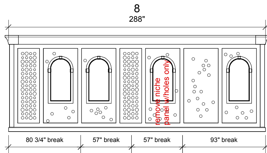
4 WEST SECTION Scale: 3/16" = 1'-0"
